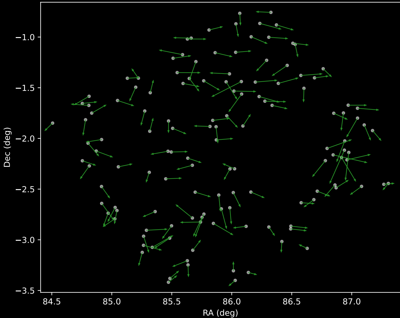
APOGEE DR17 Cluster 4 Proper Motion Vectors (n=134)
