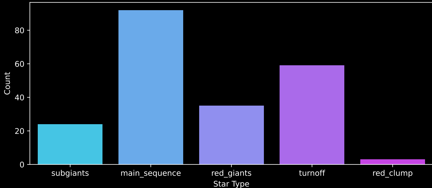
APOGEE DR17 Field: [K2_C12_072-54_btx] Count plot of Star Type
