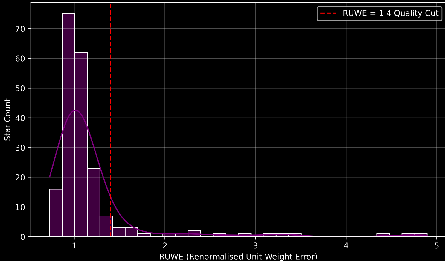
GAPOGEE DR17 Field [K2_C12_072-54_btx] RUWE Distribution (n= 202)
