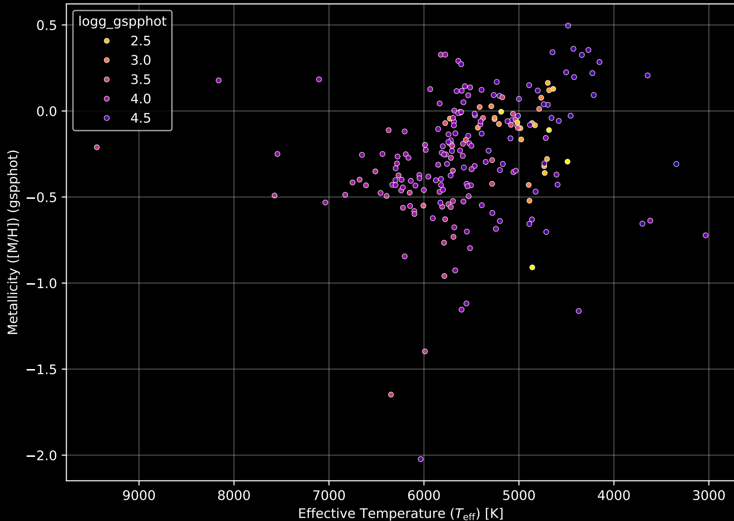
APOGEE DR17 Field: [K2_C12_072-54_btx] Stellar Population Parameters (n= 213)
