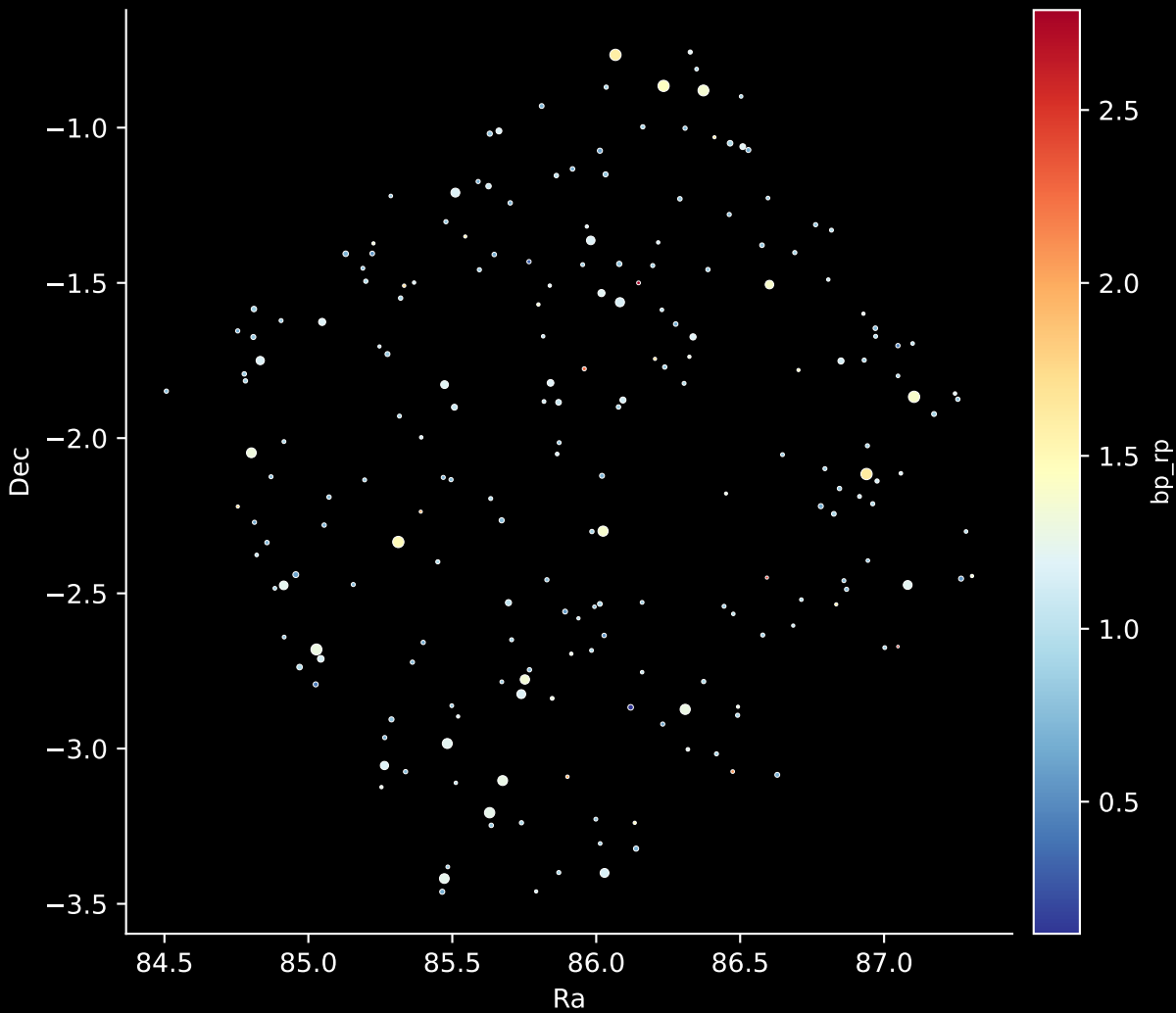
APOGEE DR17 Field: [K2_C12_072-54_btx] Stars: 213
