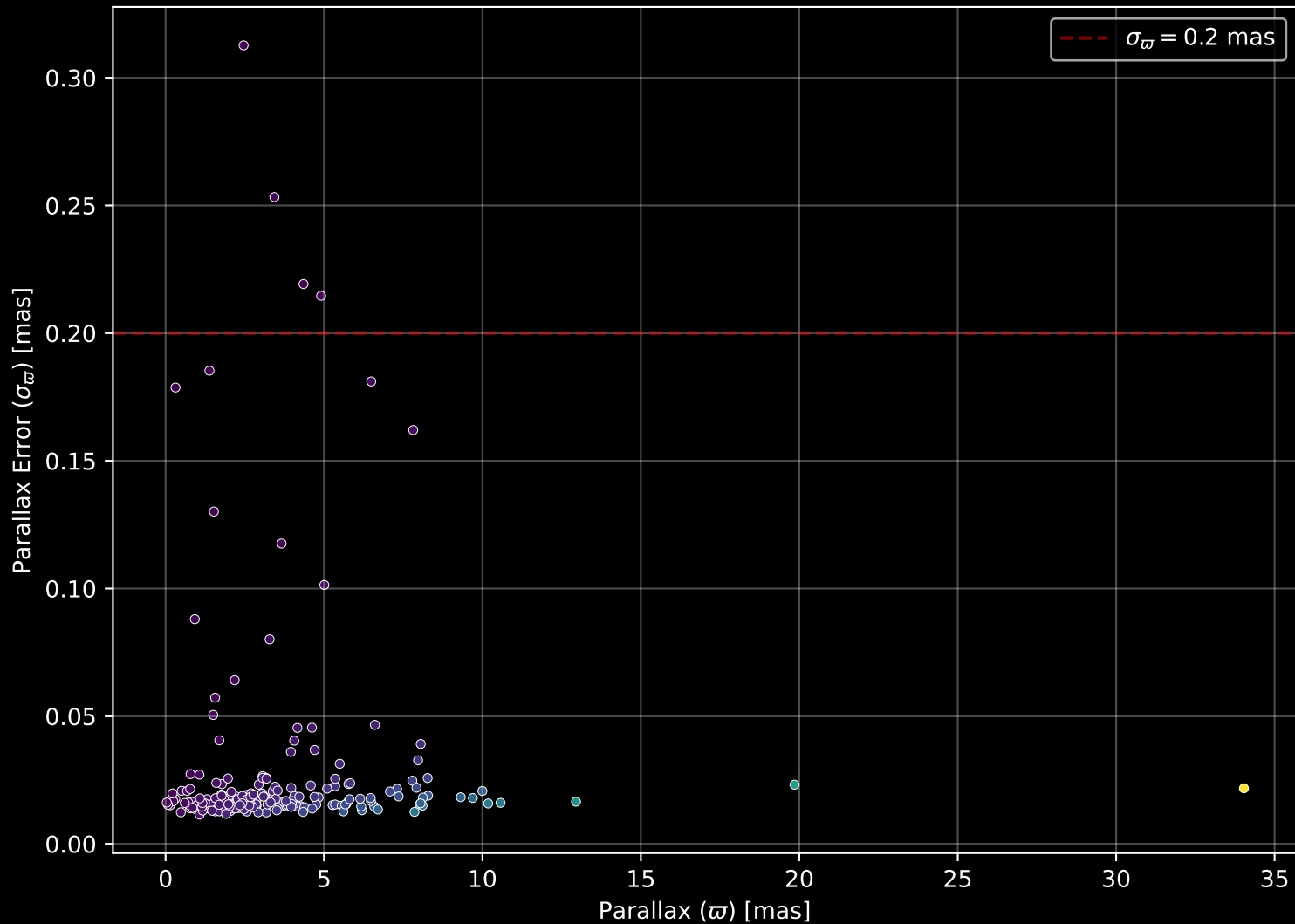
APOGEE DR17 Field: [K2_C12_072-54_btx] Parallax Quality (n= 213)
