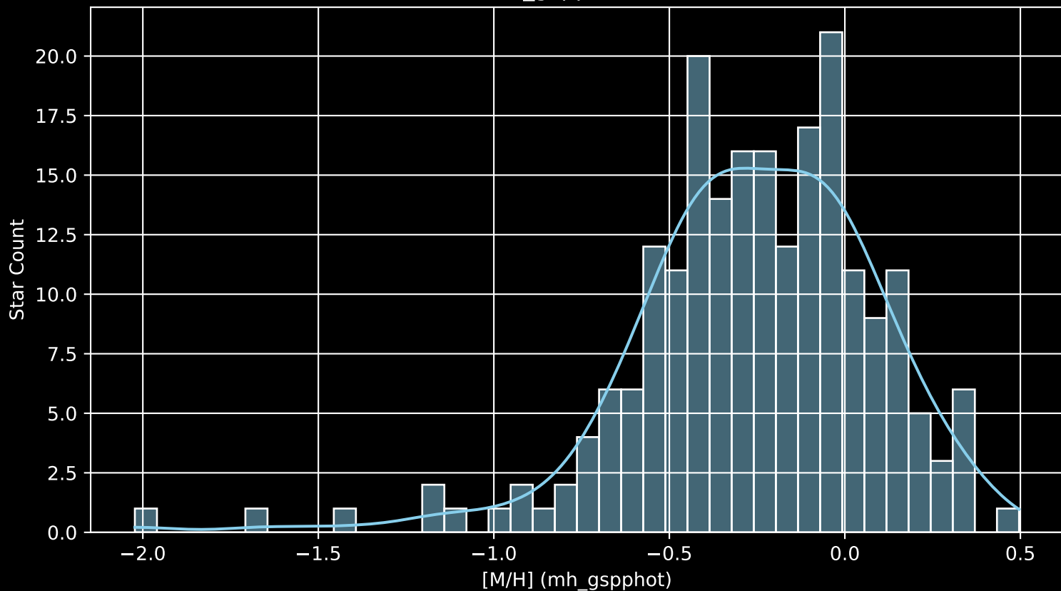
APOGEE DR17 Field: [K2_C12_072-54_btx [M/H] (mh_gspphot) (n= 213)
