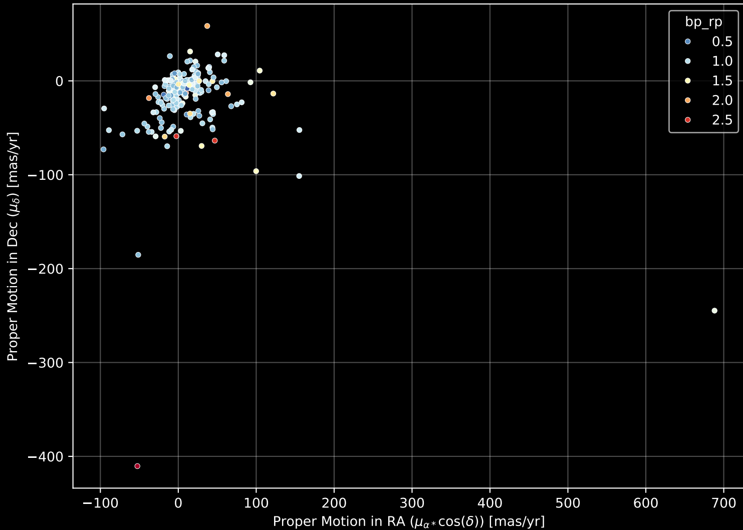
APOGEE DR17 Field: [K2_C12_072-54_btx] Proper Motion Diagram (n= 213)
